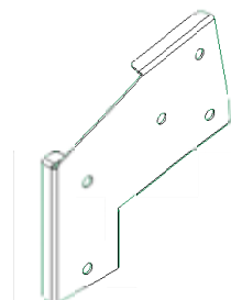
A100326 (x1) | SWING BEAM EXTENSION BRACKET-RIGHT
